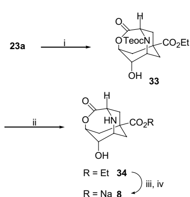
Scheme 7. Preparation of the tricyclic \epsilon -lactone, 8 , from endo epoxide, 23a . Reagents: (i) (a) \text{TMSBr} , \text{PPh}_3 , \text{CH}_2\text{Cl}_2 , -78^\circ\text{C} to rt; (b) DBU; (c) \text{HCl}/\text{H}_2\text{O} ; (ii) TBAF, KF, \text{CH}_3\text{CN} 60^\circ\text{C} ; (iii) (a) NaOH, EtOH/ \text{H}_2\text{O} ; (b) \text{HCl}/\text{H}_2\text{O} 50^\circ\text{C} .
