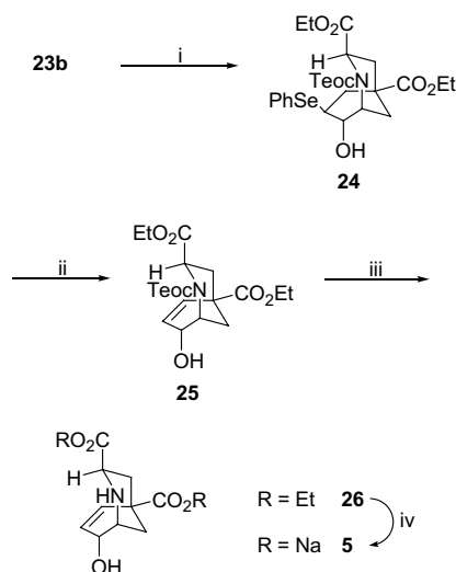
Scheme 4. Final synthetic steps and deprotections to give 5 . Reagents: (i) \text{PhSeSePh} , \text{NaBH}_4 , EtOH; (ii) (a) t -BuOOH, \text{H}_2\text{O}_2 , pyr, 0^\circ\text{C} ; (b) \text{CCl}_4 , reflux; (iii) TBAF, KF (anhyd.), \text{CH}_3\text{CN} ; (iv) NaOH, EtOH/ \text{H}_2\text{O} .
